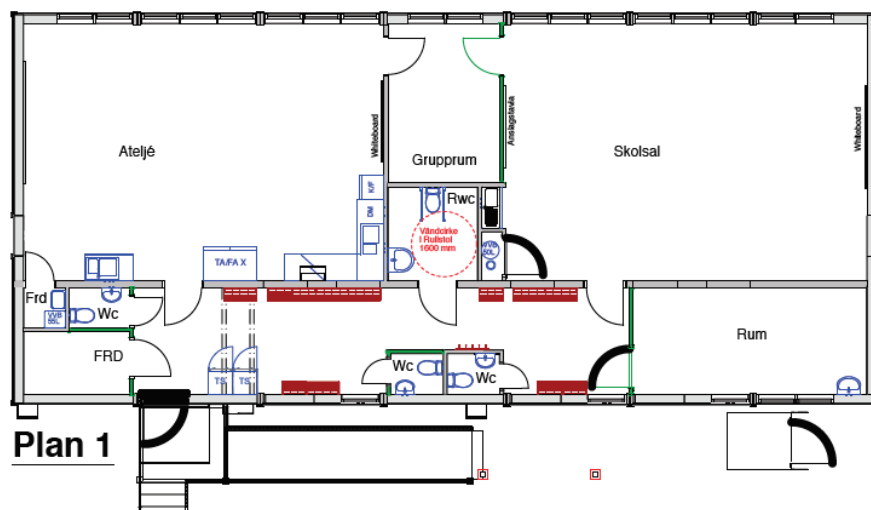
Plan 1 utformning
