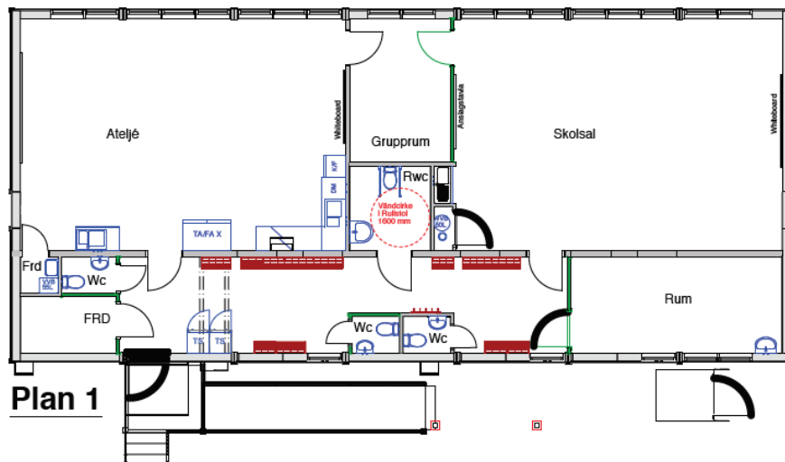
Plan 1 utformning
