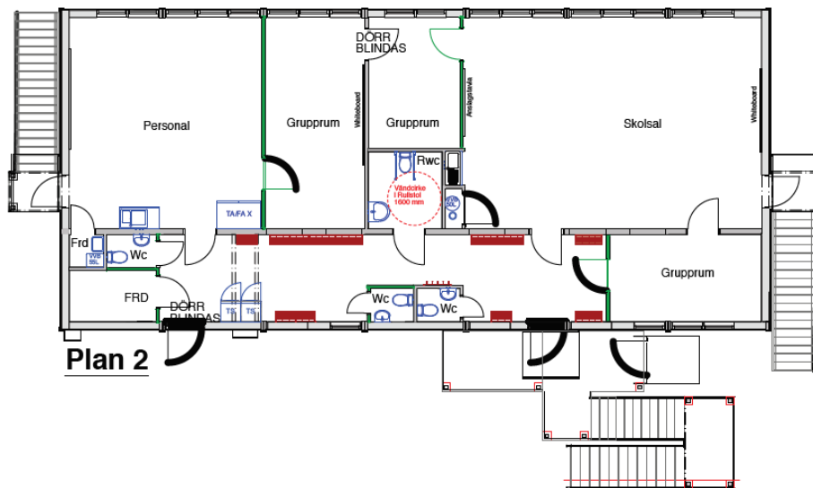
Plan 2 utformning
